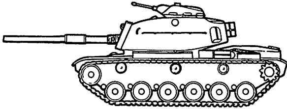
M60-UNITED STATES HIGH REAR DECK TORTOISE SHELL SHAPED TURRET 6 ROAD WHEELS WITH 3 SUPPORT ROLLERS PROMINENT CUPOLA
