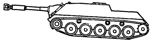
JP KANONE-WEST GERMAN NO TURRET BORE EVACUATOR AND MUZZLE BRAKE AT MUZZLE LOW FLAT-TOPPED SILHOUETTE WITH STEP BETWEEN FIGHTING COMPARTMENT AND REAR DECK 5 ROAD WHEELS WITH SUPPORT ROLLERS.
